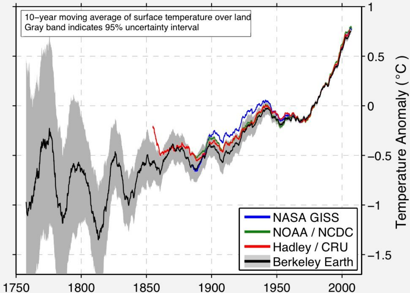
Decadal Land-Surface Average Temperature
